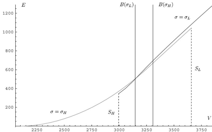
Fig. 3. Bank equity value E under value-at-risk regulation as a function of the asset value V when the bank implements the full hysteresis strategy. The vertical lines represent the closure thresholds for the low-risk and the high-risk portfolio. The two functions show the equity value for high risk ( \sigma = \sigma_H ) and low risk ( \sigma = \sigma_L ), respectively. While the bank prefers high risk when it is insolvent, it reduces risk when sufficient solvency is regained.
