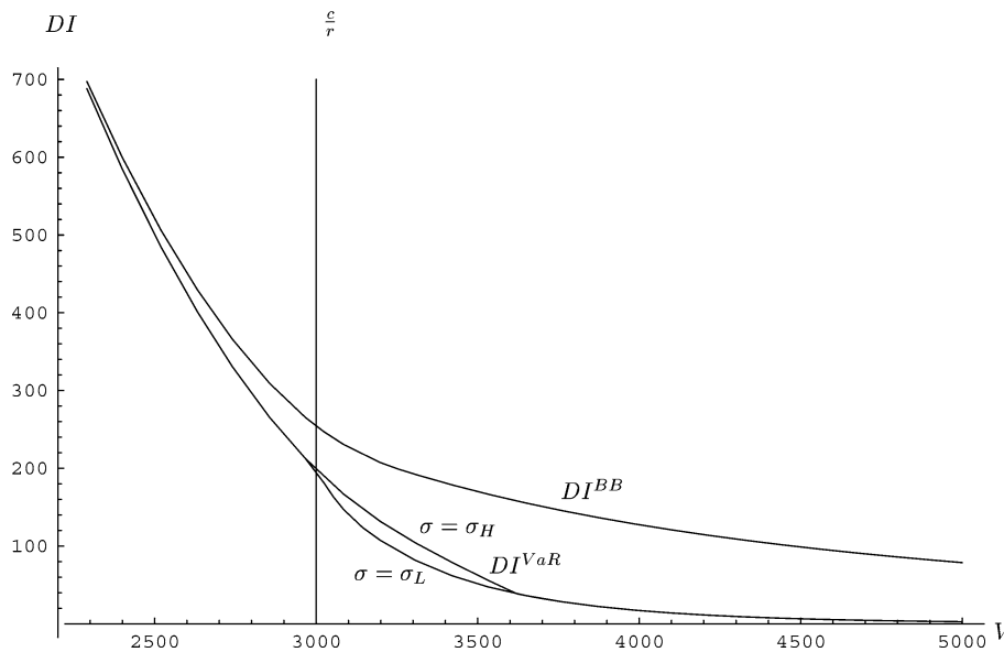
Fig. 6. The current value of the potential liability of the deposit insurance corporation for different levels of V under BB and VaR regulation. For both choices of asset risk the regulator's liability under VaR regulation is below the one under BB regulation. Under VaR regulation, the deposit insurance claim forms a hysteresis, i.e., depending on history bank managers either choose high risk \sigma_H or low risk \sigma_L .
