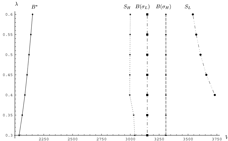
Fig. 5. Locations of the critical thresholds for the VaR regulated bank for different values of audit frequency \lambda . While the closure thresholds ( B(\cdot) ) are not affected by the auditing intensity, a tougher regulator makes it less attractive for shareholders to support an ailing bank ( B^* increases). For high audit intensities, the high-risk portfolio also becomes less attractive, managers switch earlier back to low risk ( S_L decreases). If auditing is too relaxed (here below \lambda \approx 0.37 ), bank managers do not have an incentive to switch back to low risk any more.
